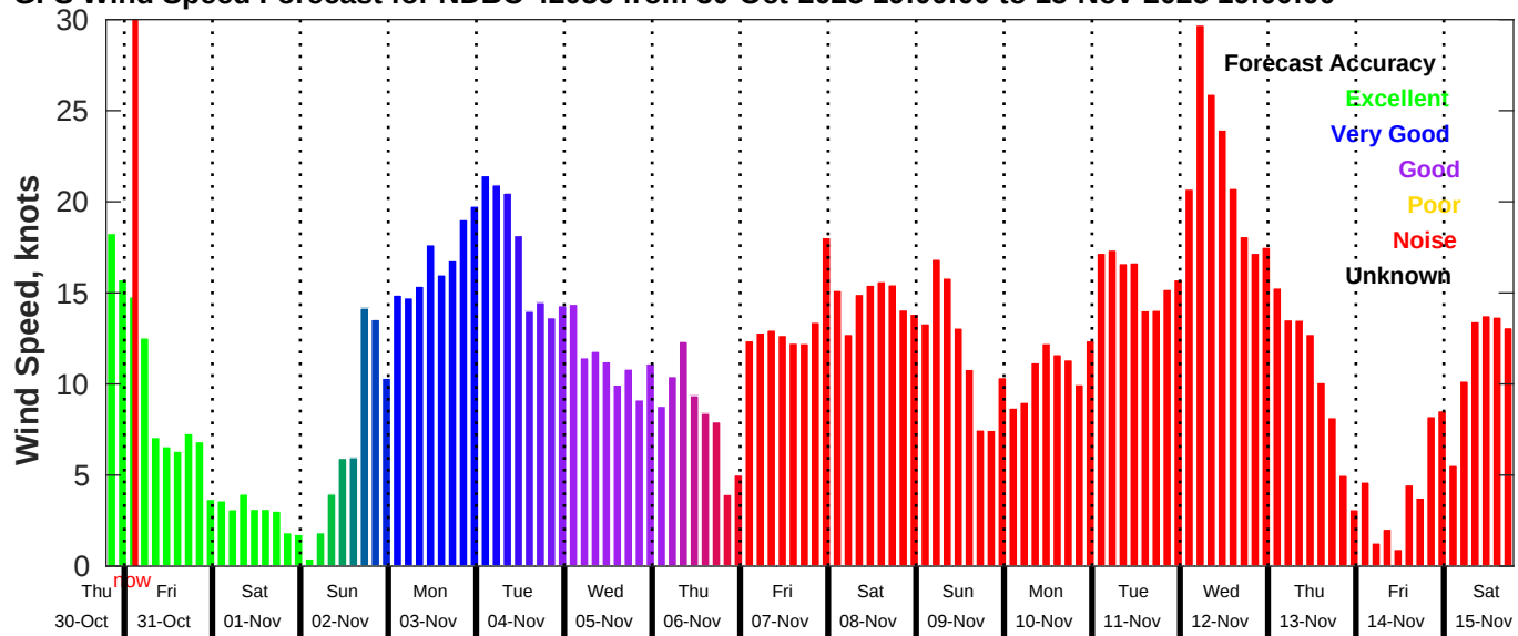
GFS Wind Speed Forecast for NDBC 42036 from 30-Oct-2025 19:00:00 to 15-Nov-2025 19:00:00
