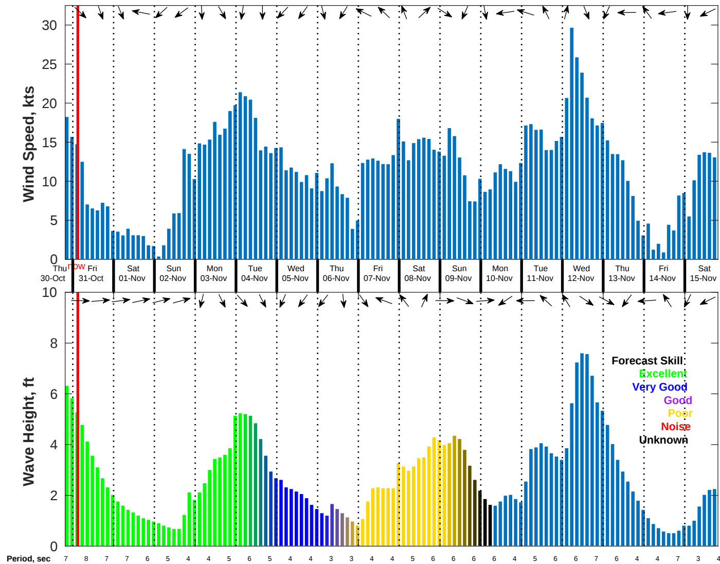
Wind & Wave Forecast for NDBC 42036 from 30-Oct-2025 19:00:00 to 15-Nov-2025 19:00:00
