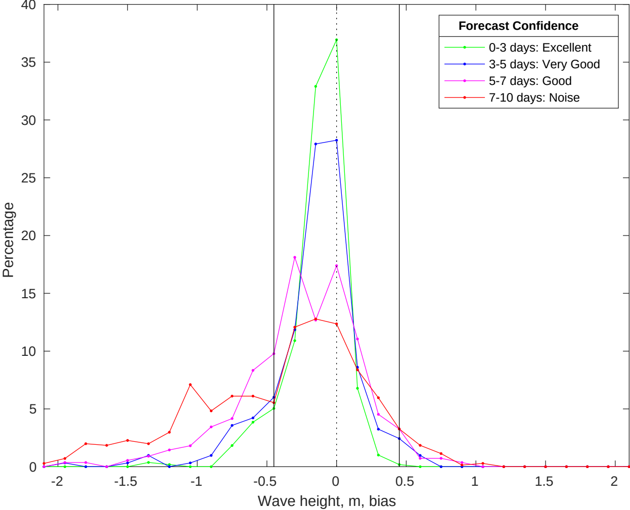
NDBC 42040 vs CMEMS Waves Bias Histogram: 31-Oct-2025
