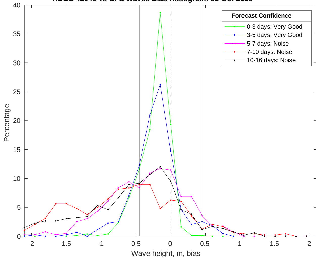
NDBC 42040 vs GFS Waves Bias Histogram: 31-Oct-2025
