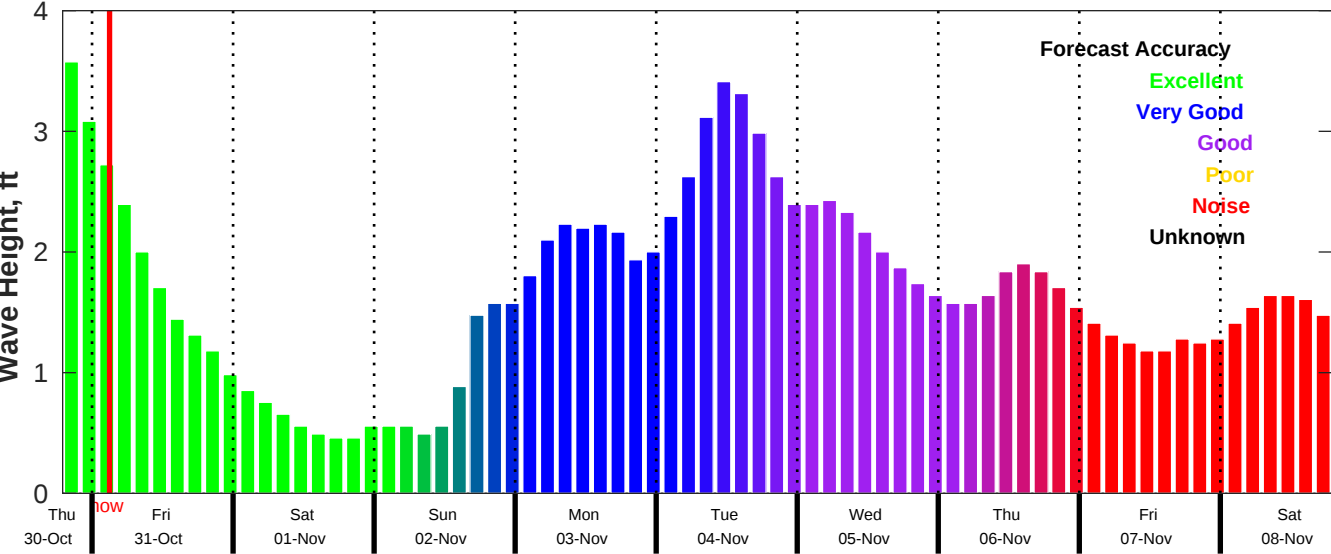
CMEMS Wave Forecast for NDBC 42040 from 30-Oct-2025 19:00:00 to 08-Nov-2025 19:00:00
