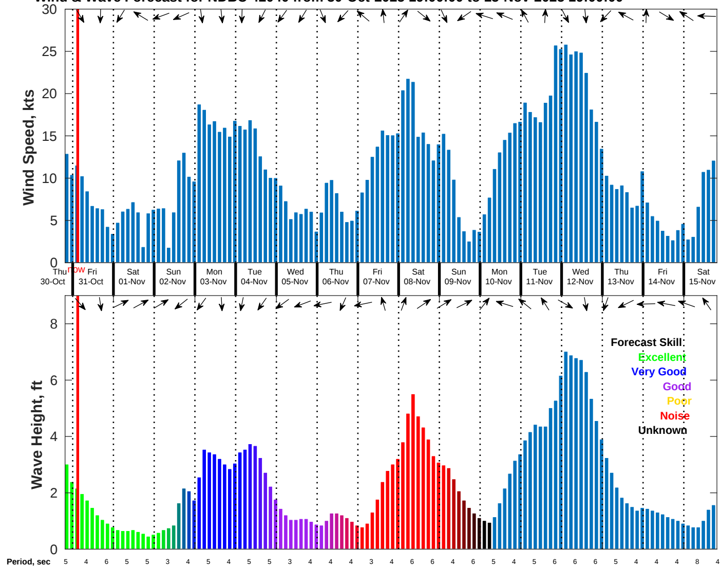
Wind & Wave Forecast for NDBC 42040 from 30-Oct-2025 19:00:00 to 15-Nov-2025 19:00:00
