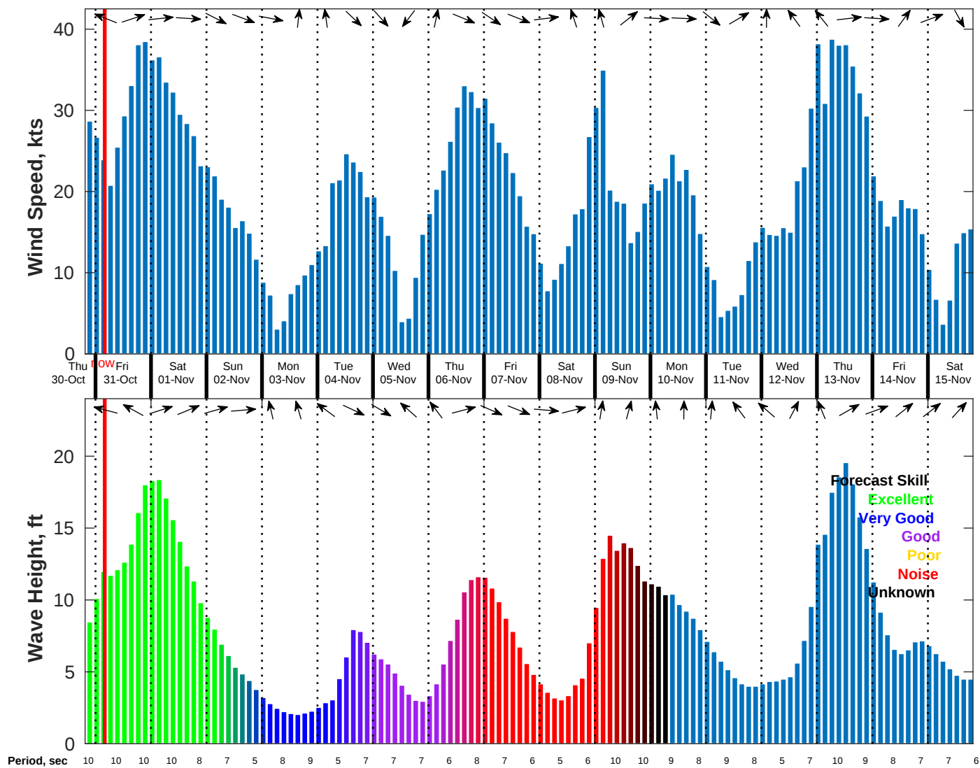
Wind & Wave Forecast for NDBC 44008 from 30-Oct-2025 20:00:00 to 15-Nov-2025 20:00:00
