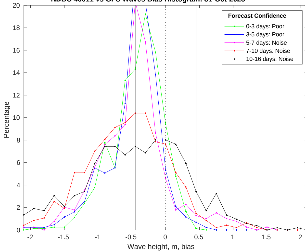
NDBC 46011 vs GFS Waves Bias Histogram: 31-Oct-2025
