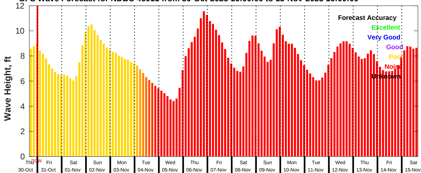
GFS Wave Forecast for NDBC 46011 from 30-Oct-2025 16:00:00 to 15-Nov-2025 16:00:00
