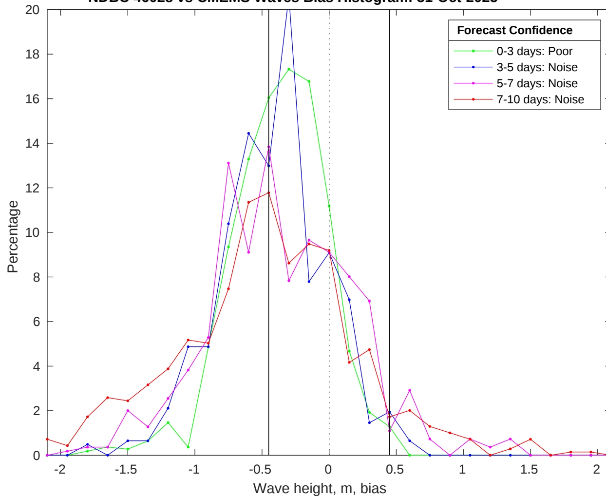
NDBC 46028 vs CMEMS Waves Bias Histogram: 31-Oct-2025
