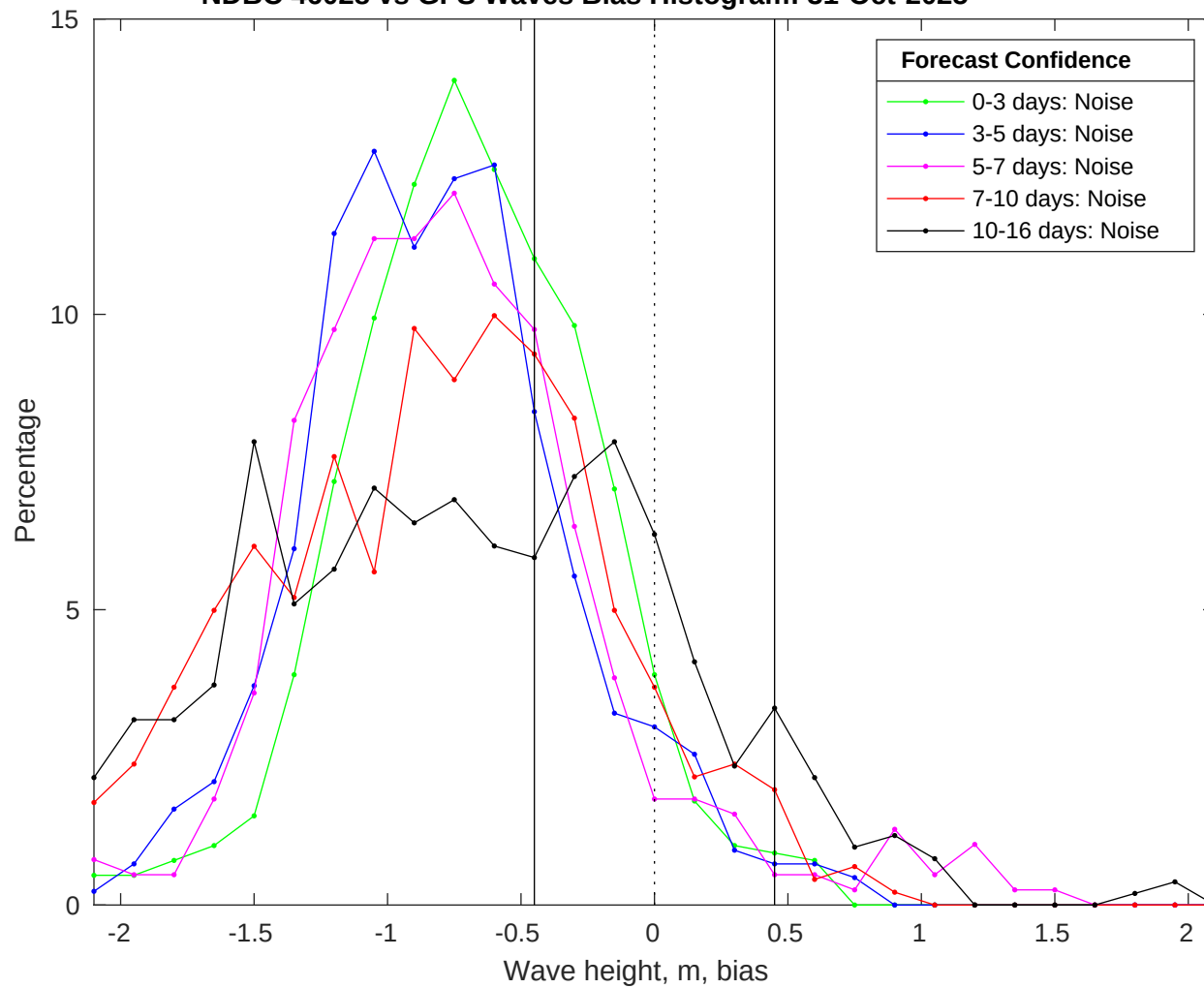
NDBC 46028 vs GFS Waves Bias Histogram: 31-Oct-2025
