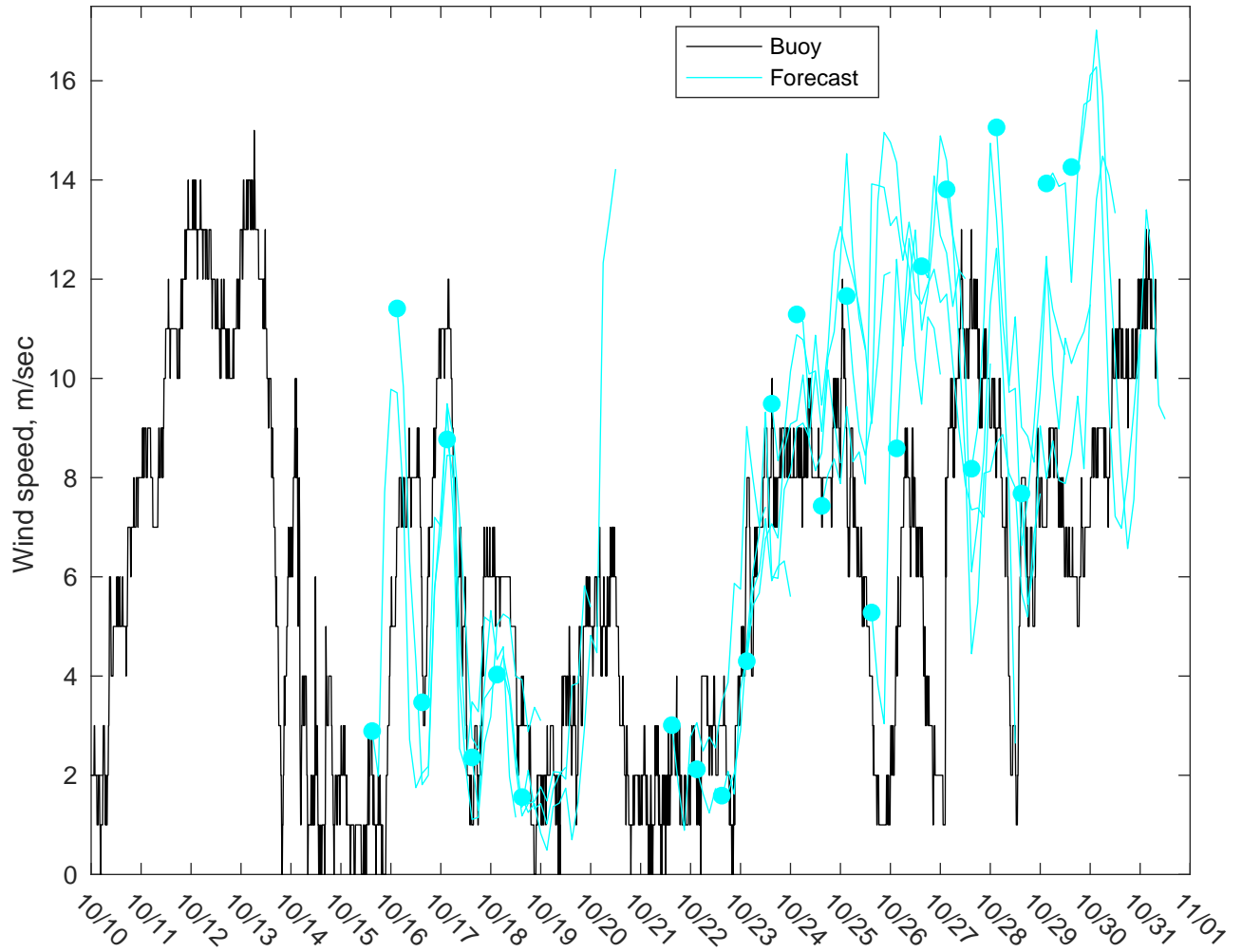
NDBC 46028 vs GFS Winds: 5 to 7 day forecast
