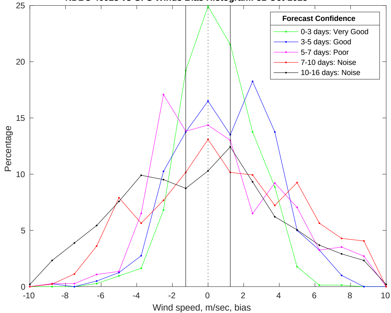
NDBC 46028 vs GFS Winds Bias Histogram: 31-Oct-2025
