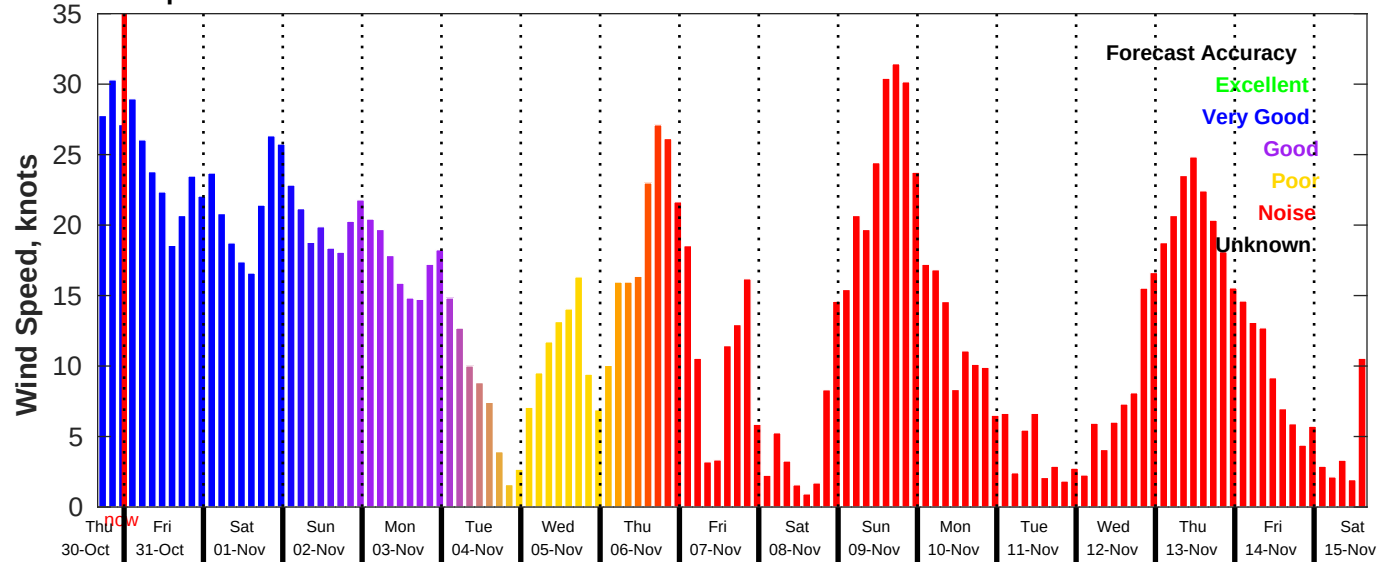
GFS Wind Speed Forecast for NDBC 46028 from 30-Oct-2025 16:00:00 to 15-Nov-2025 16:00:00
