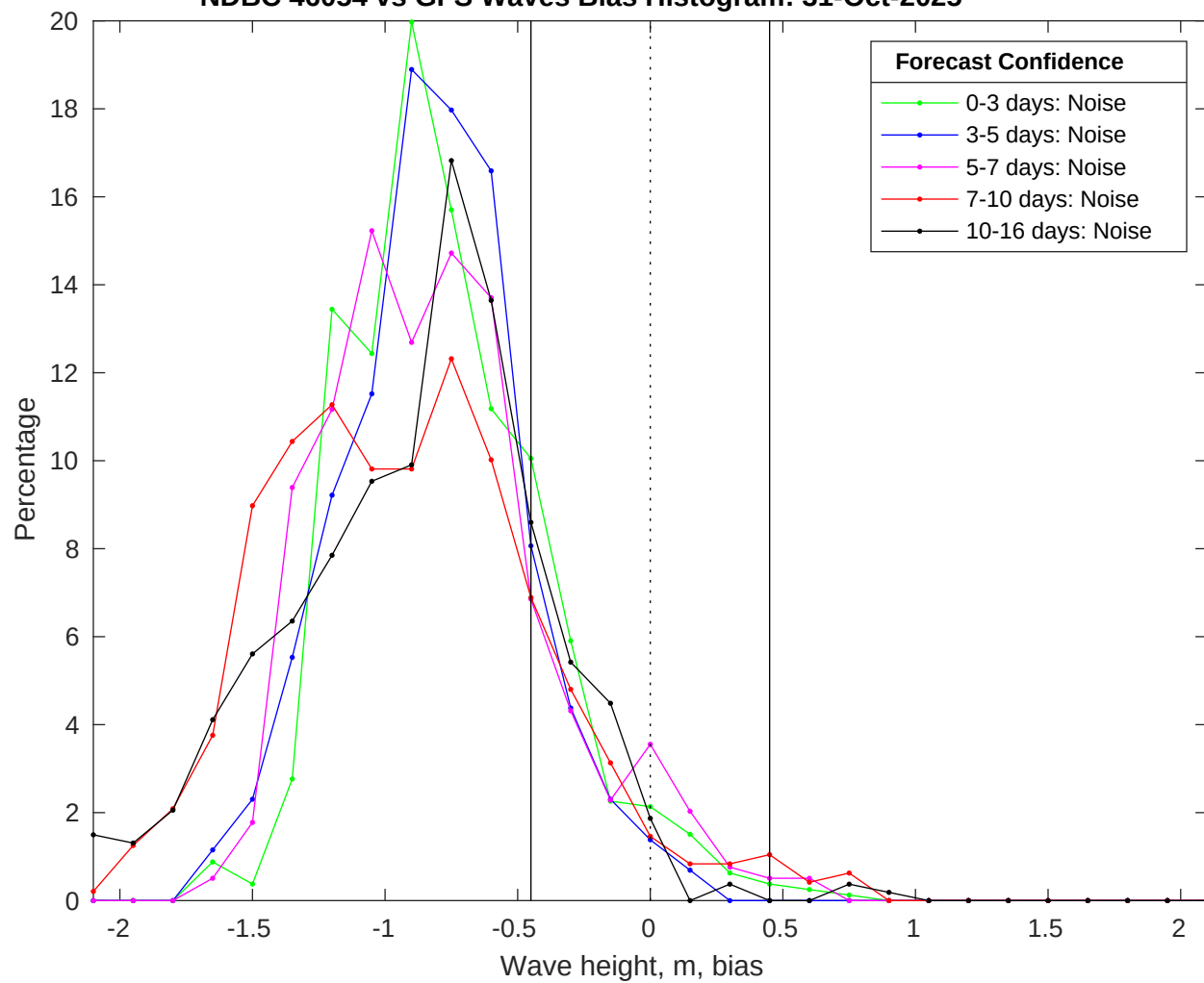
NDBC 46054 vs GFS Waves Bias Histogram: 31-Oct-2025
