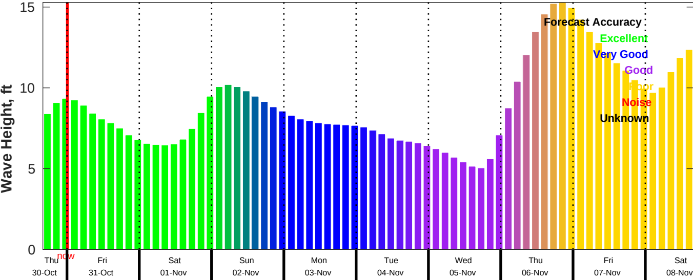
CMEMS Wave Forecast for NDBC 46054 from 30-Oct-2025 16:00:00 to 08-Nov-2025 16:00:00
