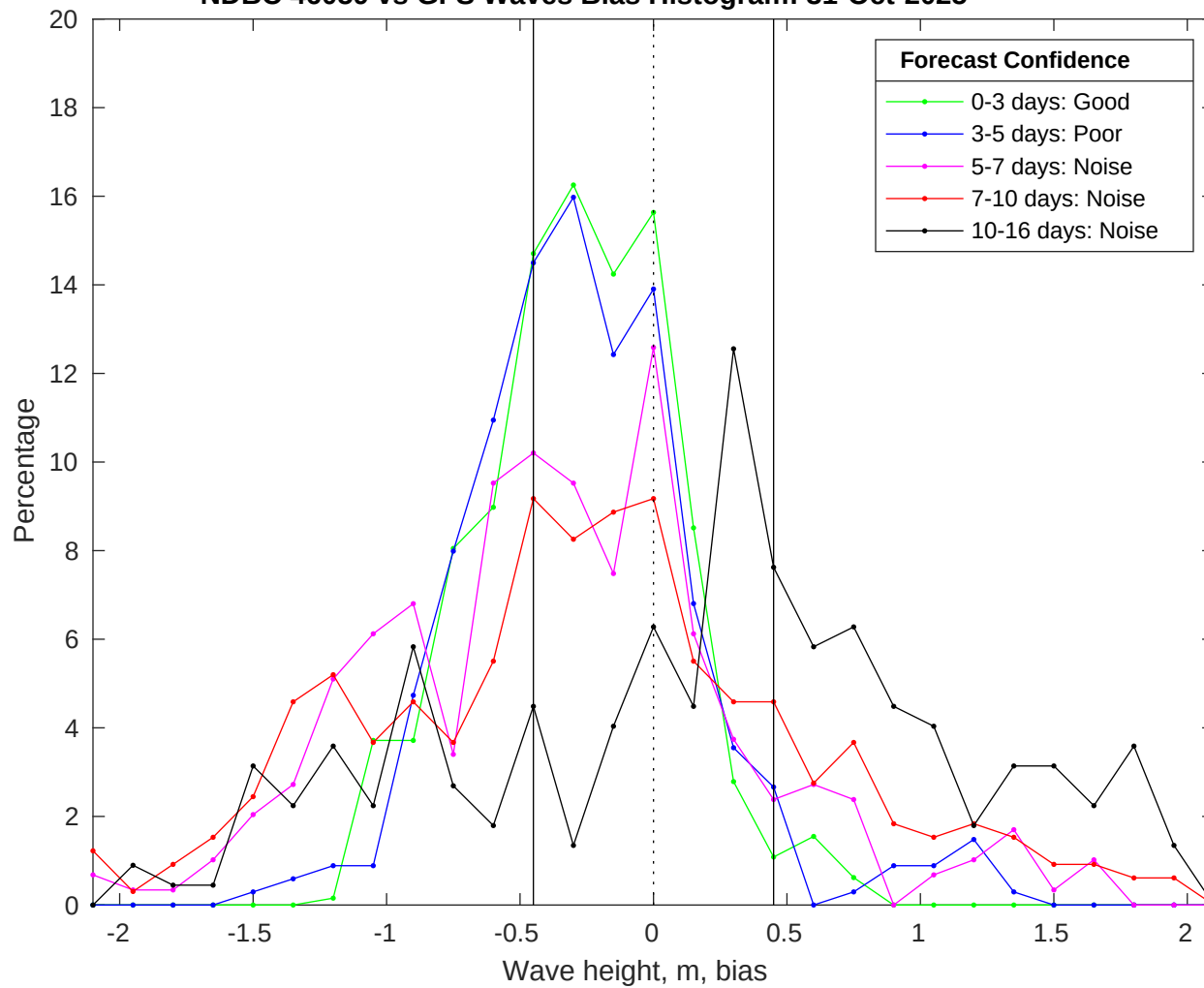
NDBC 46059 vs GFS Waves Bias Histogram: 31-Oct-2025
