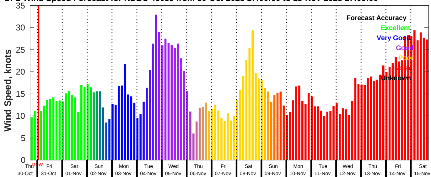
GFS Wind Speed Forecast for NDBC 46059 from 30-Oct-2025 17:00:00 to 15-Nov-2025 17:00:00
