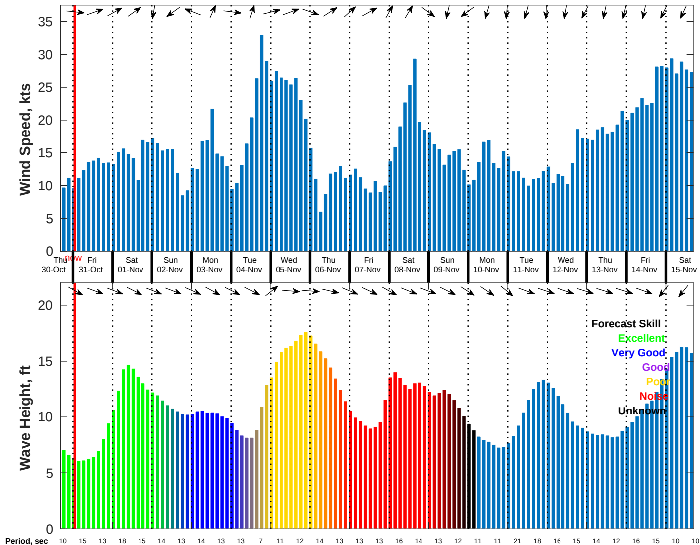
Wind & Wave Forecast for NDBC 46059 from 30-Oct-2025 17:00:00 to 15-Nov-2025 17:00:00
