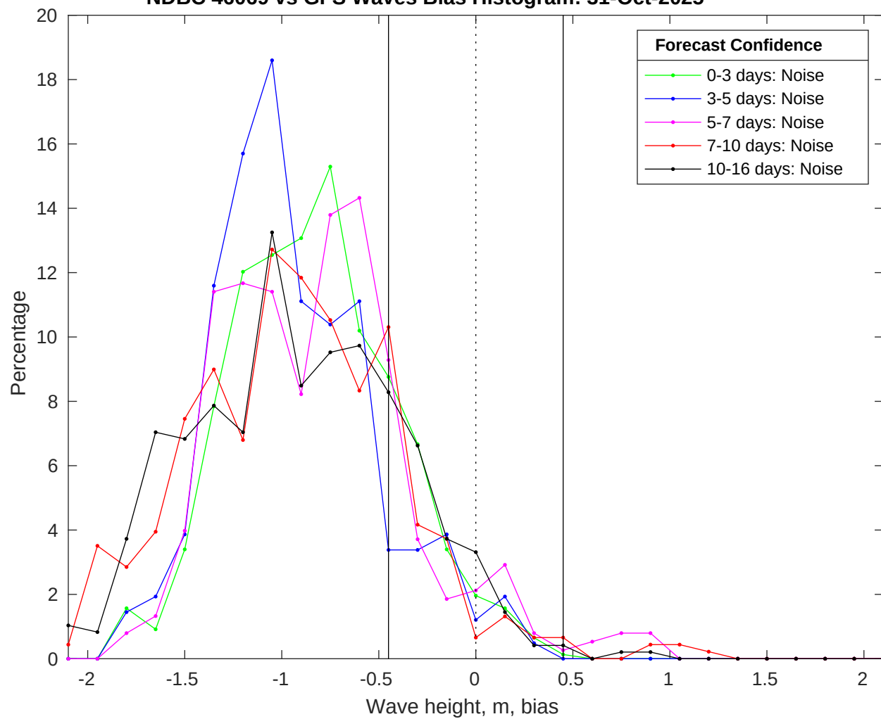
NDBC 46069 vs GFS Waves Bias Histogram: 31-Oct-2025
