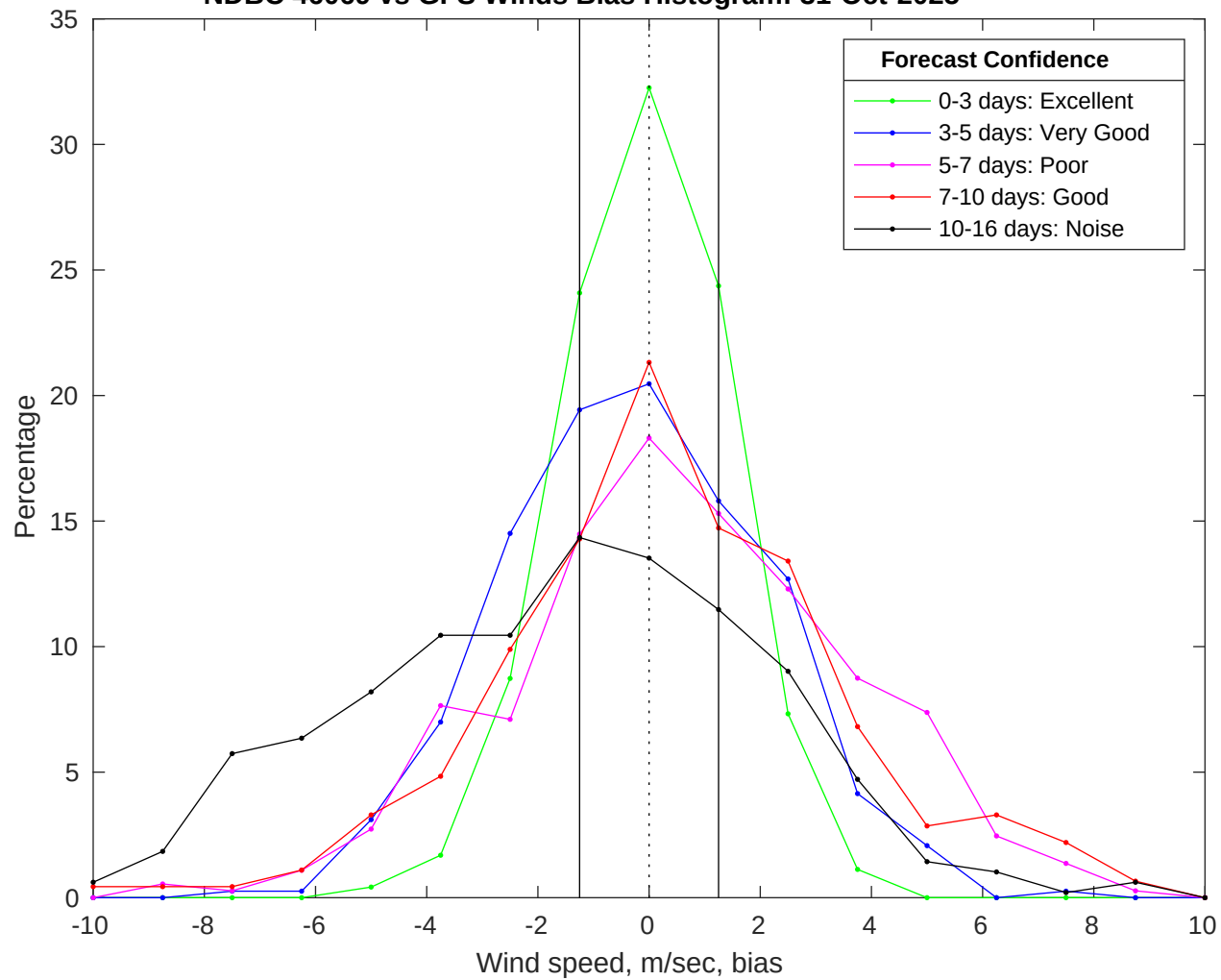
NDBC 46069 vs GFS Winds Bias Histogram: 31-Oct-2025
