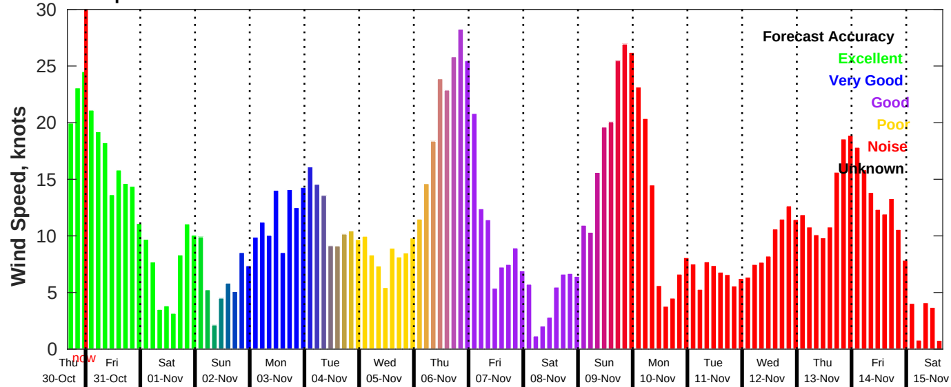
GFS Wind Speed Forecast for NDBC 46069 from 30-Oct-2025 16:00:00 to 15-Nov-2025 16:00:00
