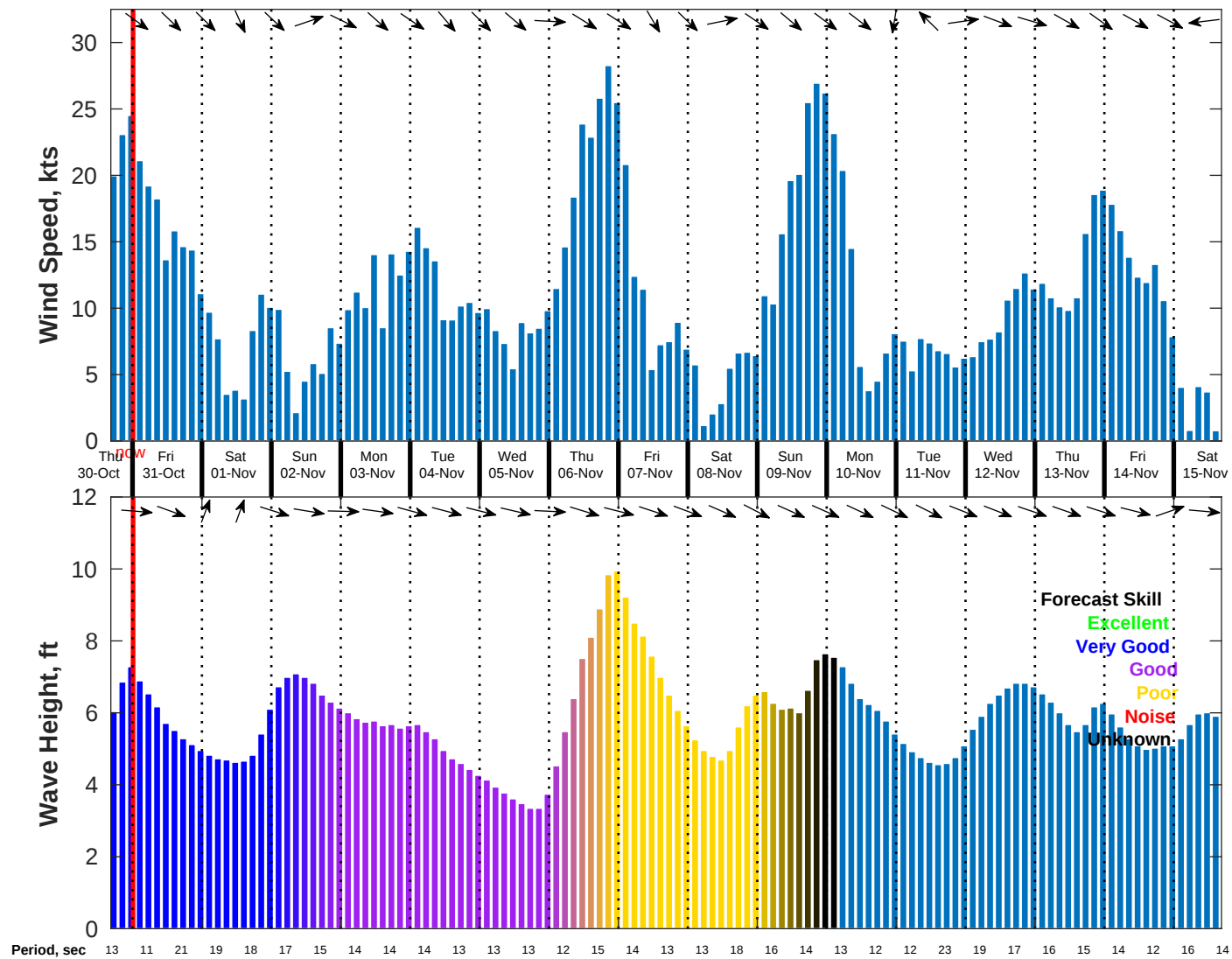
Wind & Wave Forecast for NDBC 46069 from 30-Oct-2025 16:00:00 to 15-Nov-2025 16:00:00
