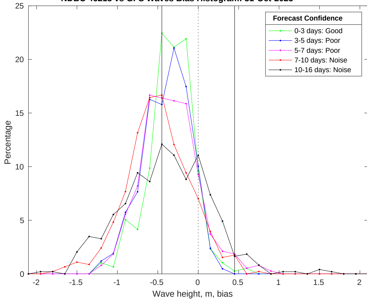
NDBC 46215 vs GFS Waves Bias Histogram: 31-Oct-2025
