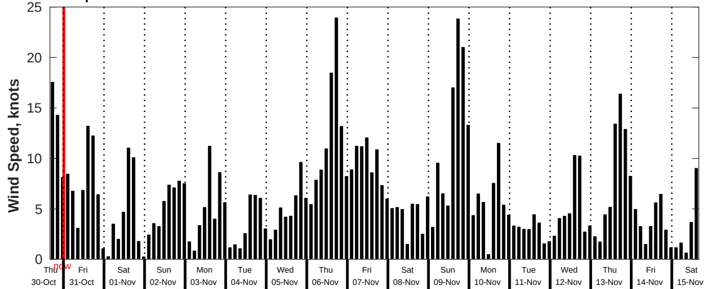
GFS Wind Speed Forecast for NDBC 46215 from 30-Oct-2025 16:00:00 to 15-Nov-2025 16:00:00
