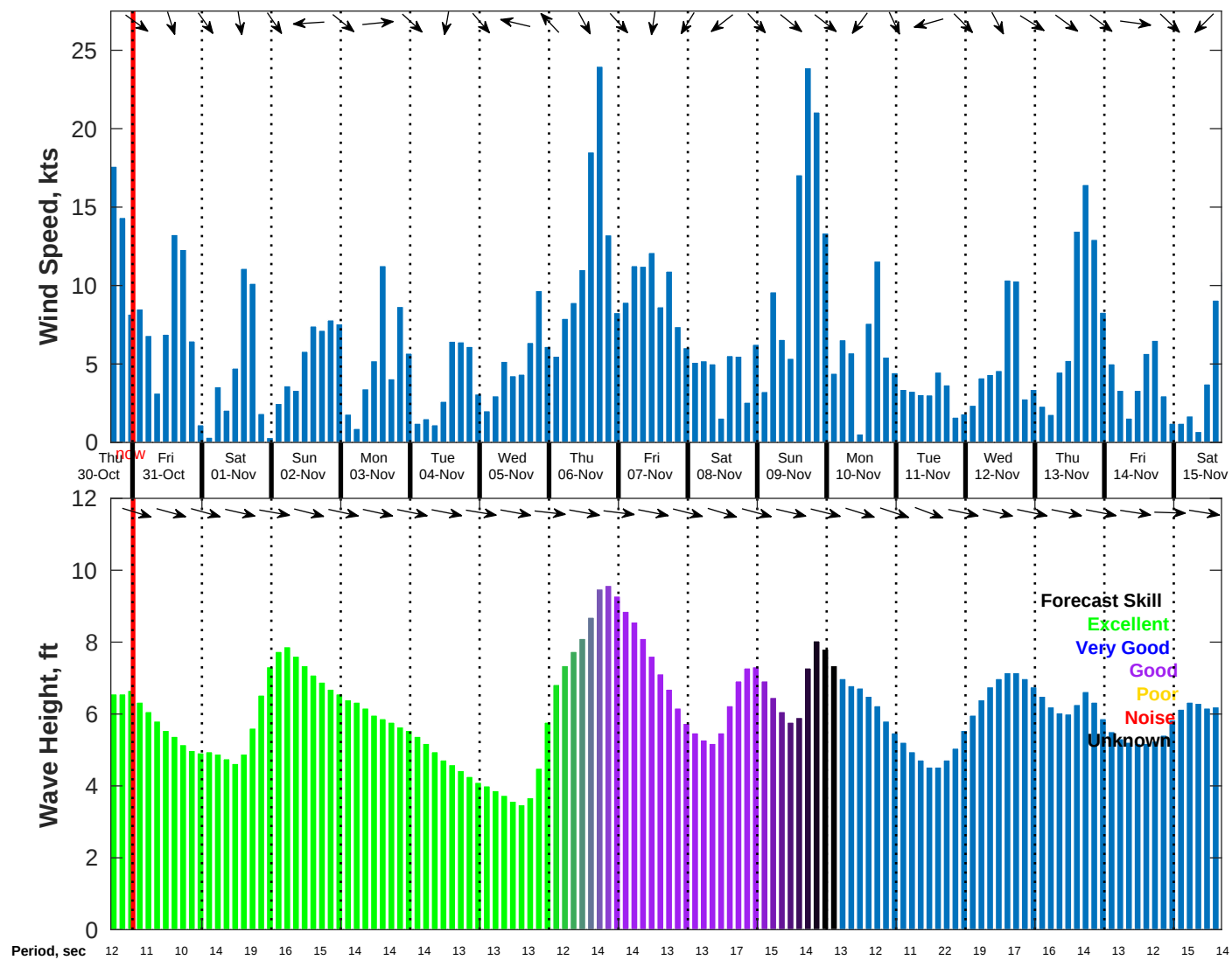
Wind & Wave Forecast for NDBC 46215 from 30-Oct-2025 16:00:00 to 15-Nov-2025 16:00:00
