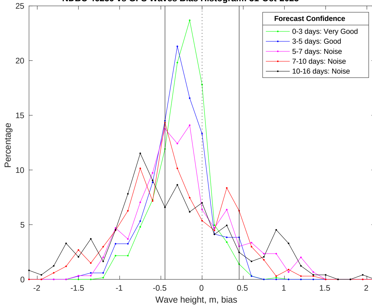
NDBC 46259 vs GFS Waves Bias Histogram: 31-Oct-2025
