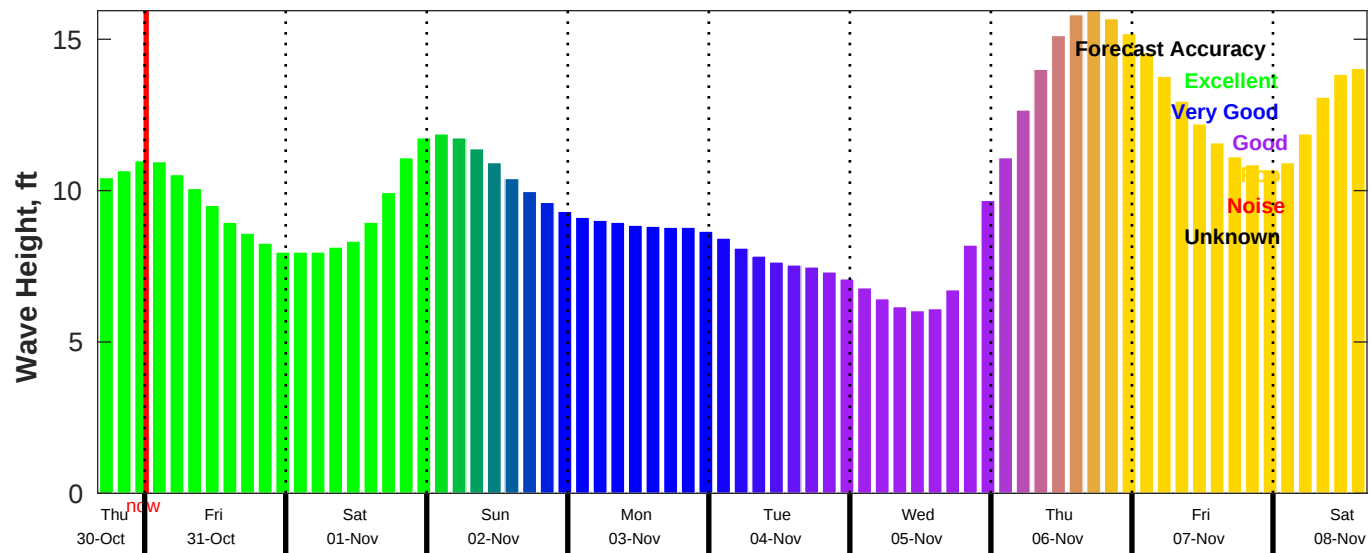
CMEMS Wave Forecast for NDBC 46259 from 30-Oct-2025 16:00:00 to 08-Nov-2025 16:00:00
