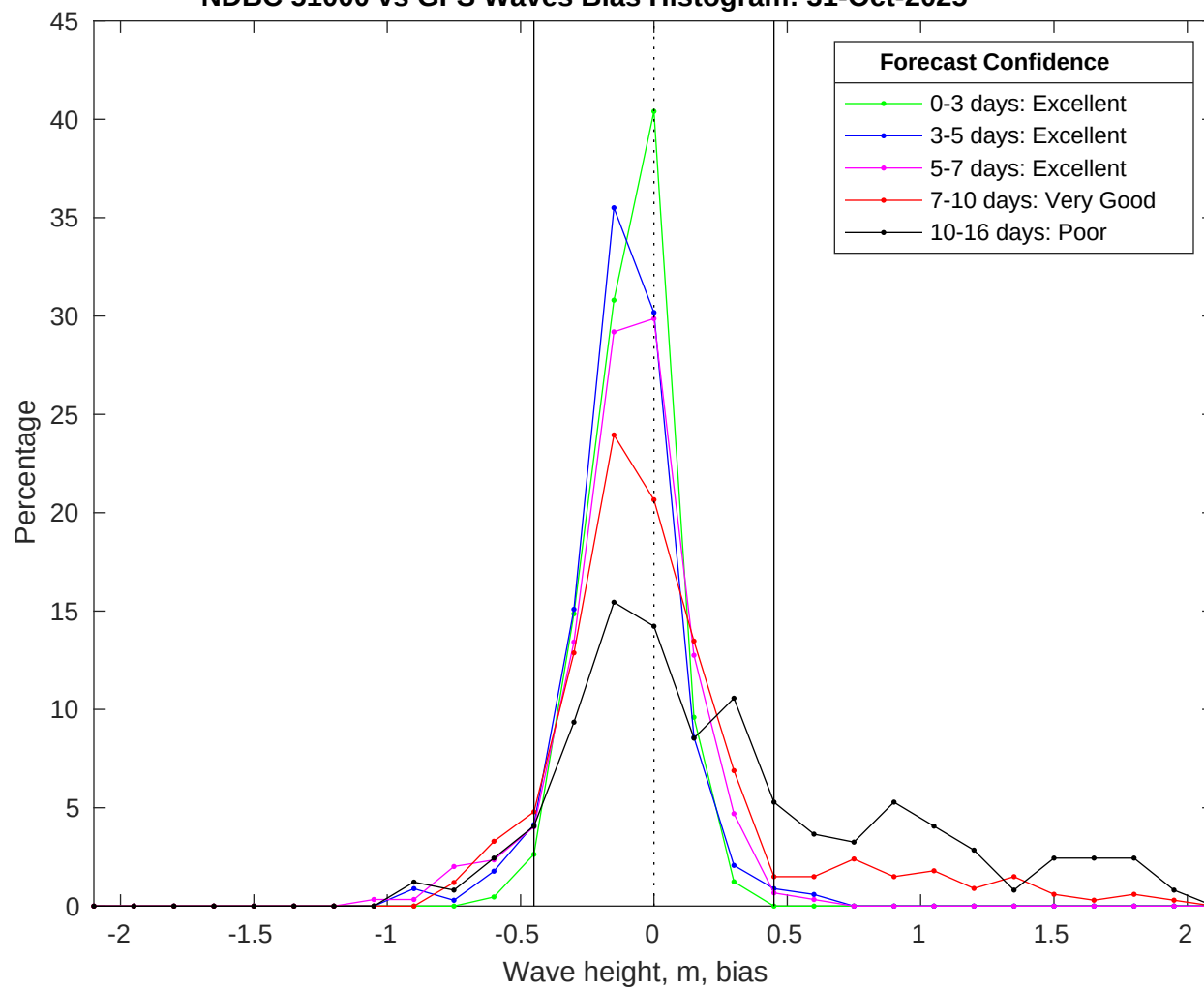
NDBC 51000 vs GFS Waves Bias Histogram: 31-Oct-2025
