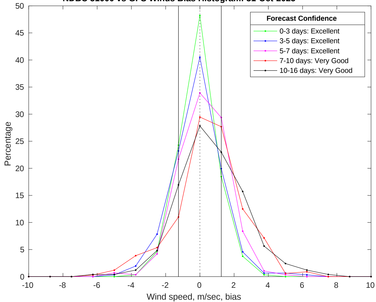
NDBC 51000 vs GFS Winds Bias Histogram: 31-Oct-2025
