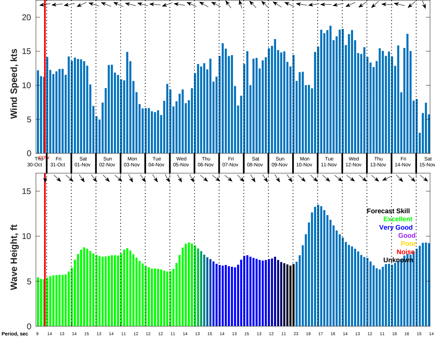
Wind & Wave Forecast for NDBC 51000 from 30-Oct-2025 14:00:00 to 15-Nov-2025 14:00:00
