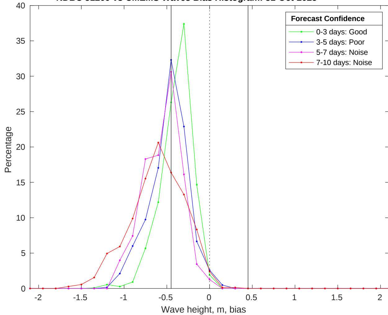
NDBC 51209 vs CMEMS Waves Bias Histogram: 31-Oct-2025
