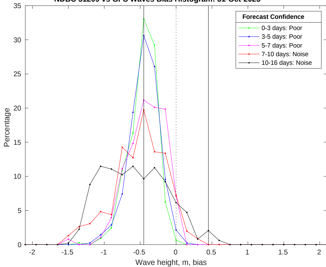
NDBC 51209 vs GFS Waves Bias Histogram: 31-Oct-2025
