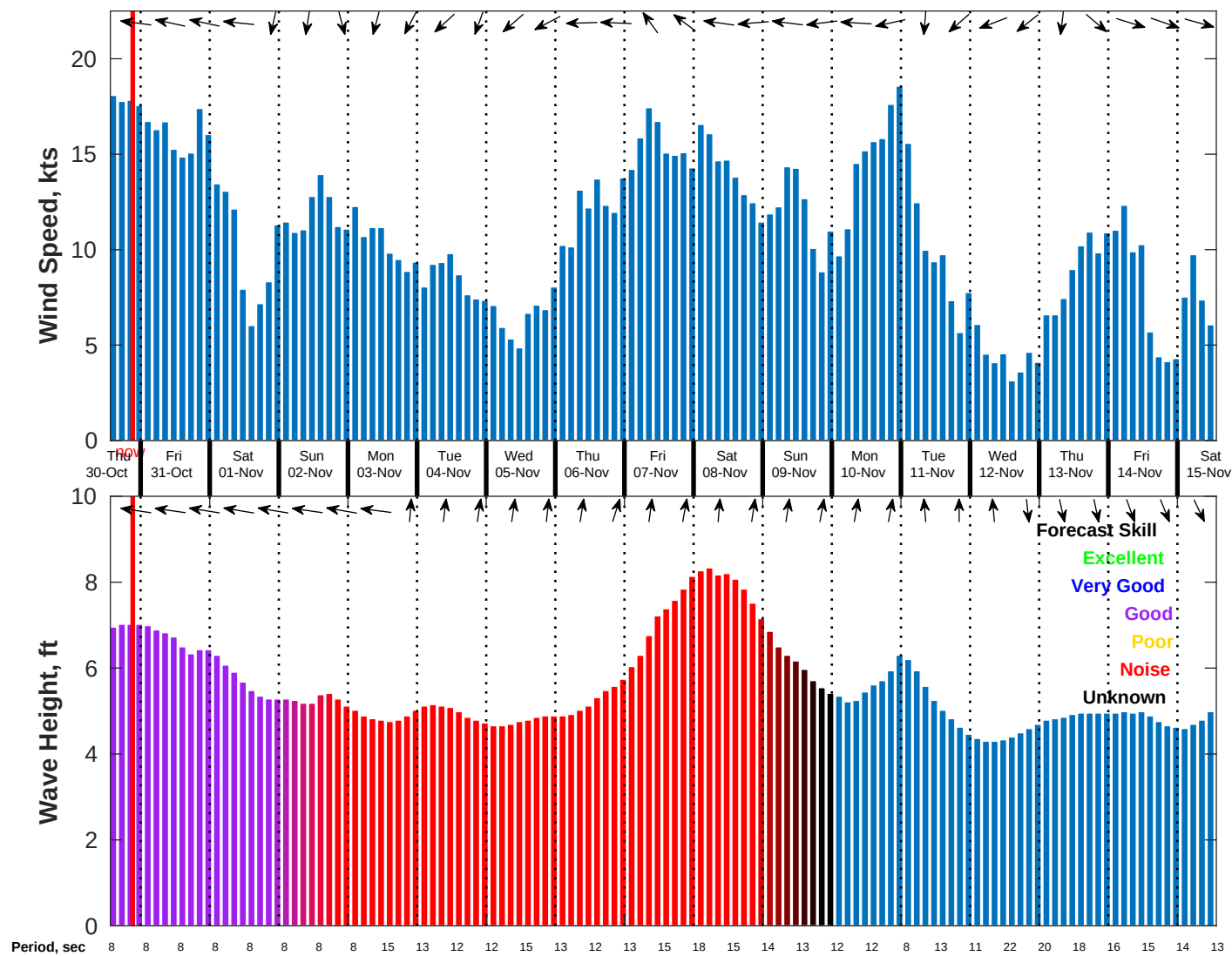
Wind & Wave Forecast for NDBC 51209 from 30-Oct-2025 13:00:00 to 15-Nov-2025 13:00:00
