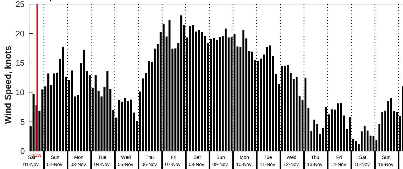
GFS Wind Speed Forecast for NDBC 52212 from 31-Oct-2025 09:00:00 to 16-Nov-2025 09:00:00
