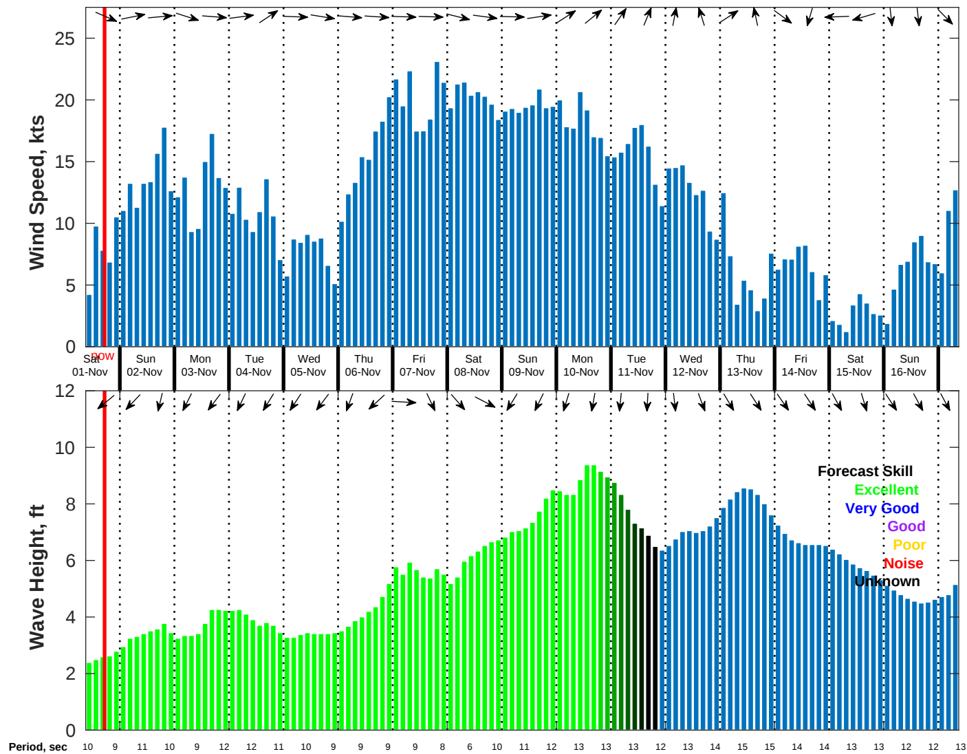
Wind & Wave Forecast for NDBC 52212 from 31-Oct-2025 09:00:00 to 16-Nov-2025 09:00:00
