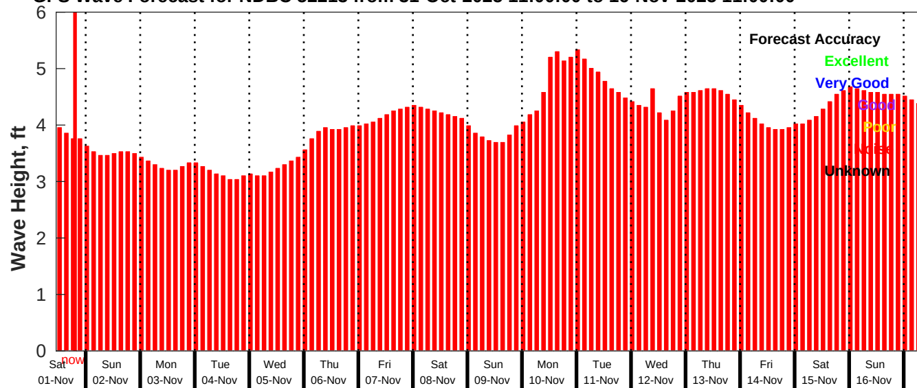
GFS Wave Forecast for NDBC 52213 from 31-Oct-2025 11:00:00 to 16-Nov-2025 11:00:00
