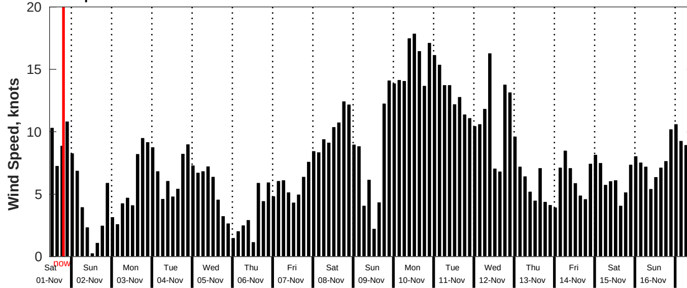
GFS Wind Speed Forecast for NDBC 52213 from 31-Oct-2025 11:00:00 to 16-Nov-2025 11:00:00
