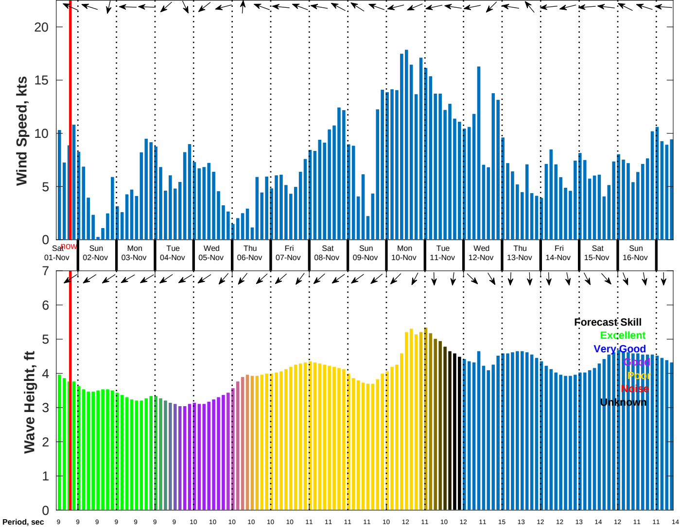
Wind & Wave Forecast for NDBC 52213 from 31-Oct-2025 11:00:00 to 16-Nov-2025 11:00:00
