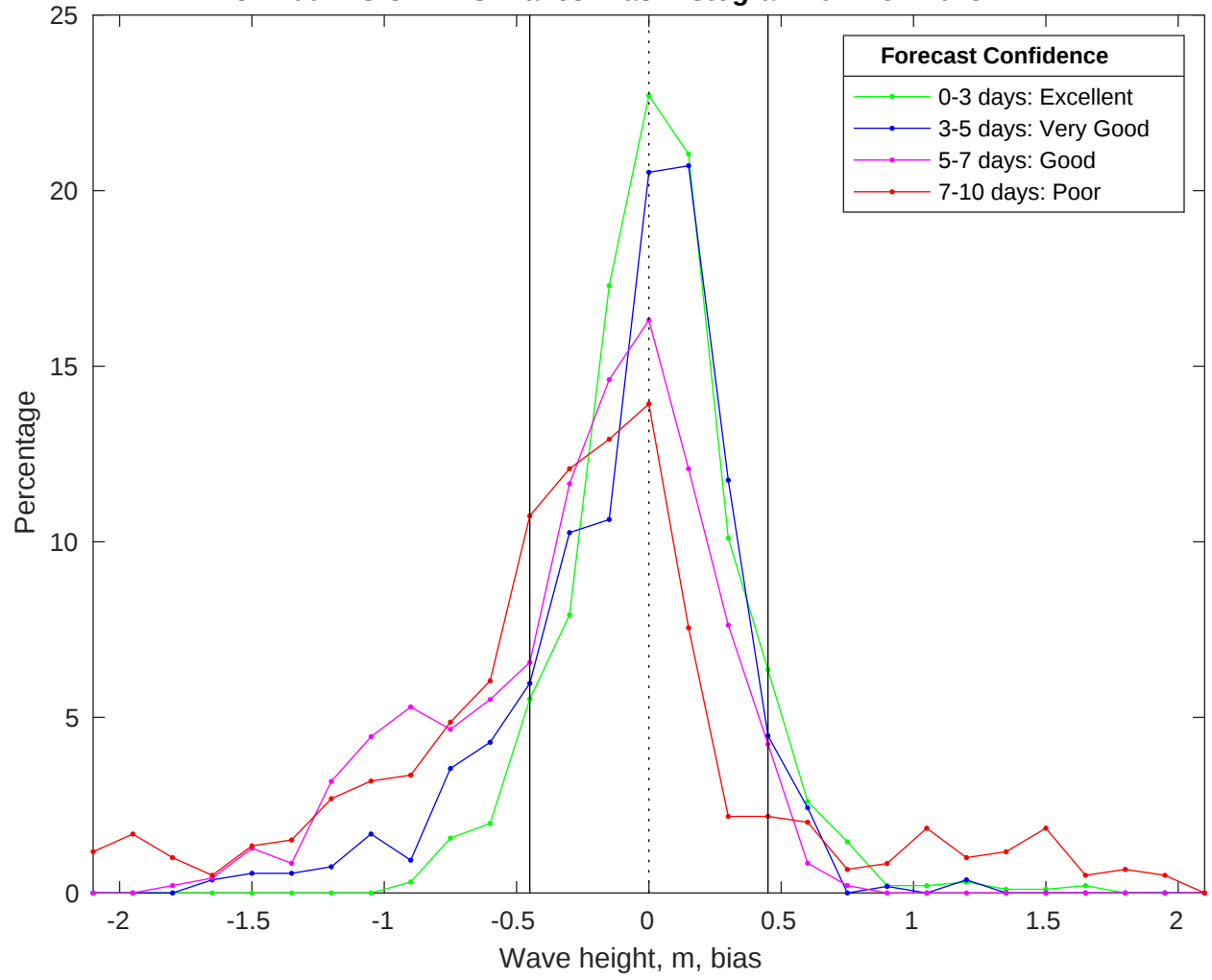
NDBC 41004 vs CMEMS Waves Bias Histogram: 01-Nov-2025
