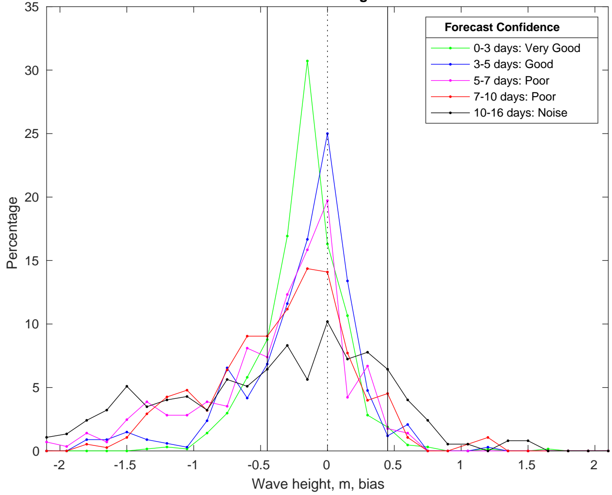
NDBC 41004 vs GFS Waves Bias Histogram: 01-Nov-2025
