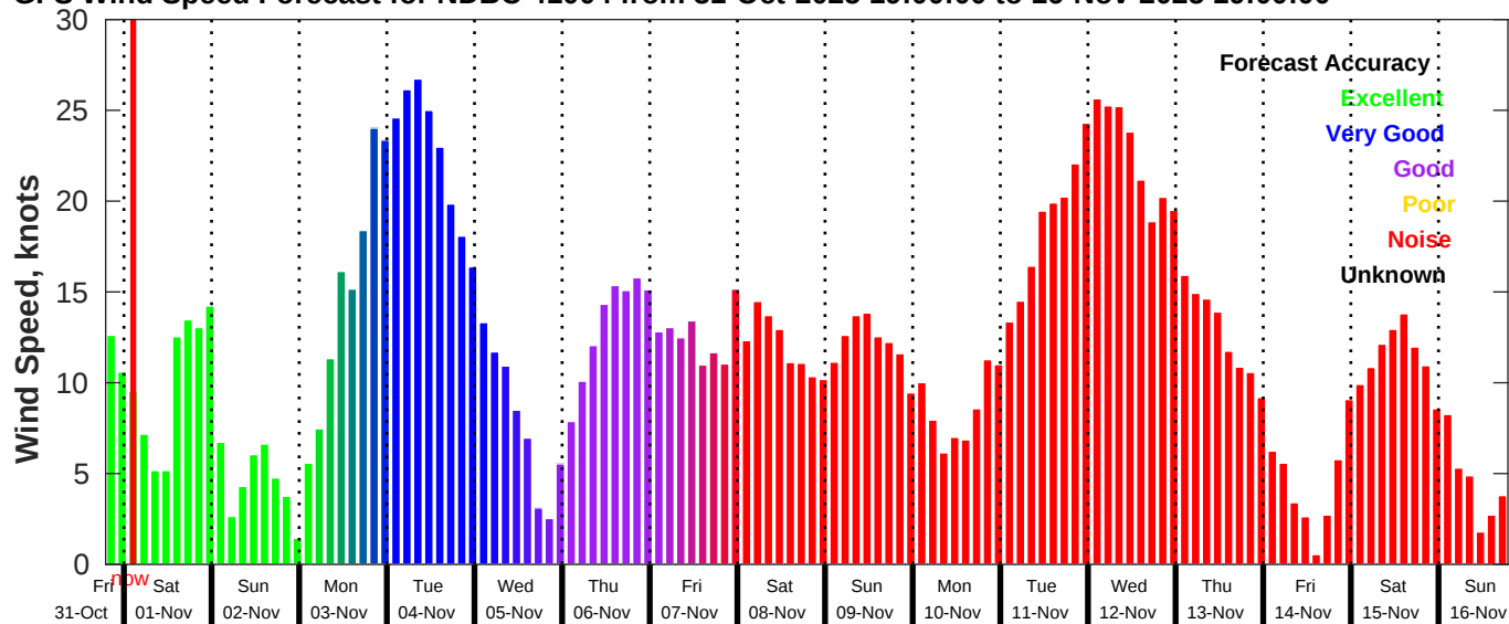
GFS Wind Speed Forecast for NDBC 41004 from 31-Oct-2025 19:00:00 to 16-Nov-2025 19:00:00
