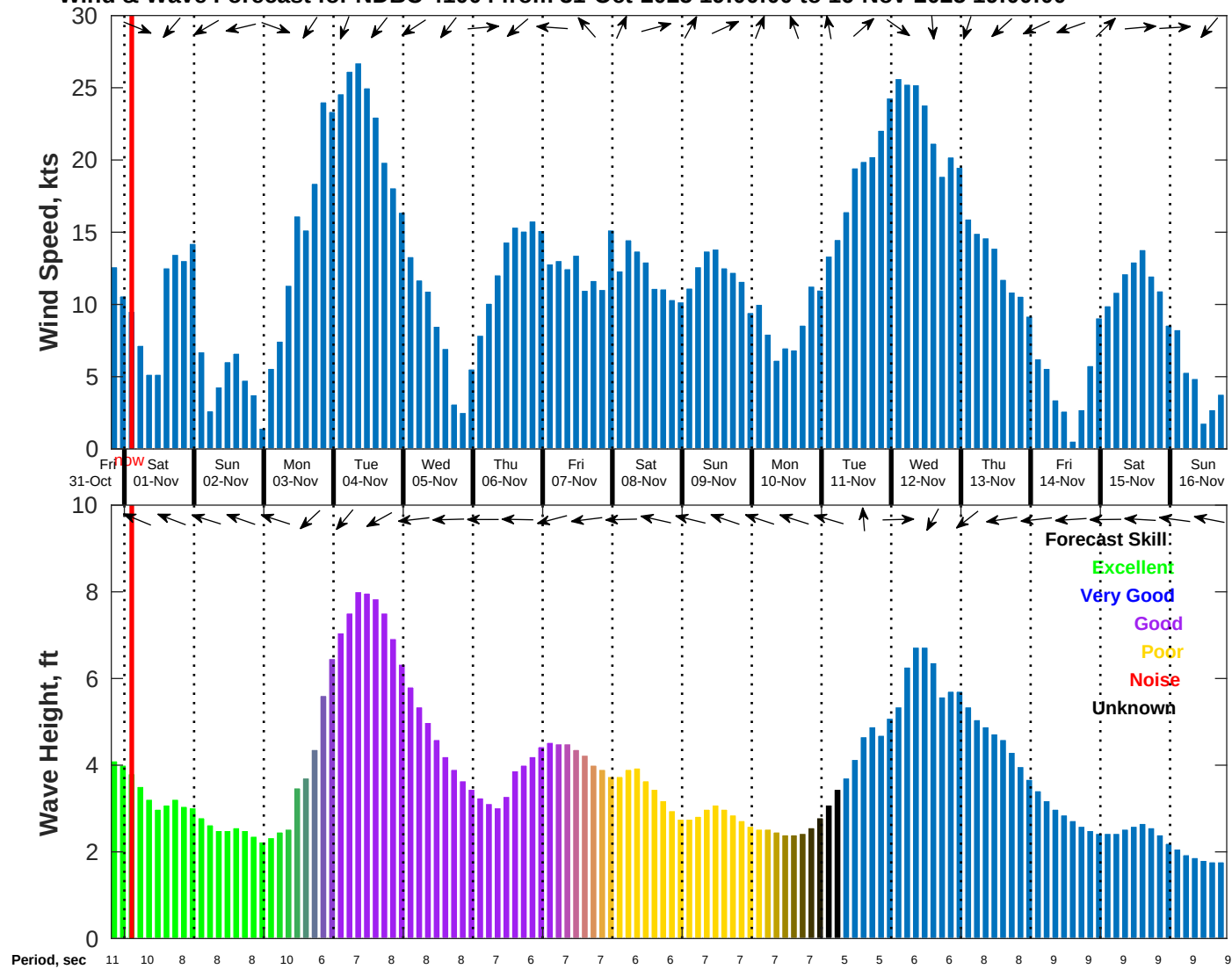
Wind & Wave Forecast for NDBC 41004 from 31-Oct-2025 19:00:00 to 16-Nov-2025 19:00:00
