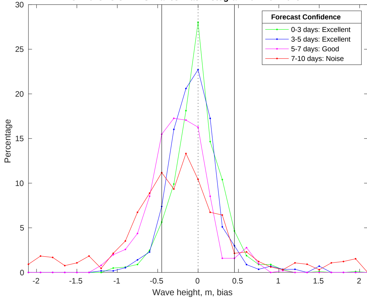
NDBC 41013 vs CMEMS Waves Bias Histogram: 01-Nov-2025
