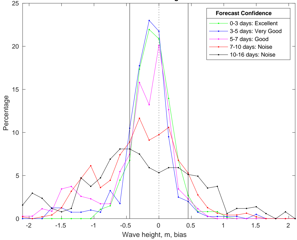
NDBC 41013 vs GFS Waves Bias Histogram: 01-Nov-2025
