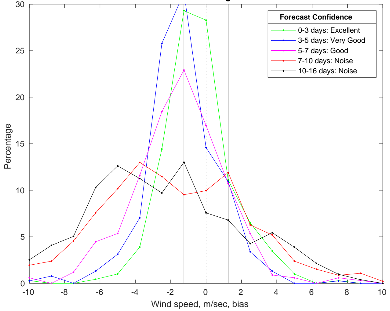
NDBC 41013 vs GFS Winds Bias Histogram: 01-Nov-2025
