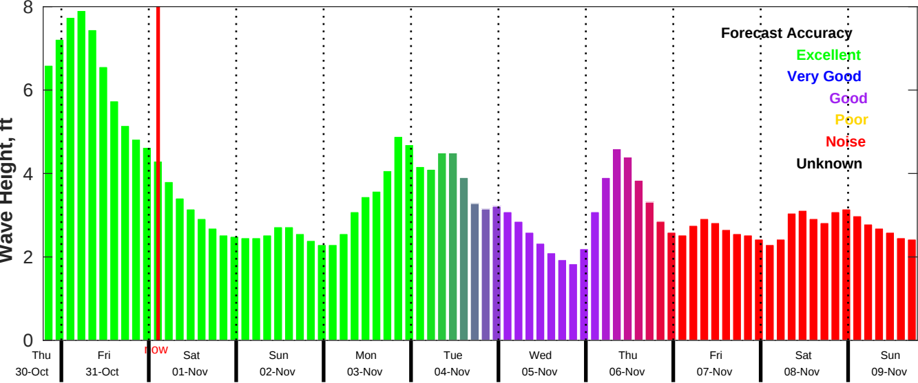
CMEMS Wave Forecast for NDBC 41013 from 30-Oct-2025 19:00:00 to 09-Nov-2025 19:00:00
