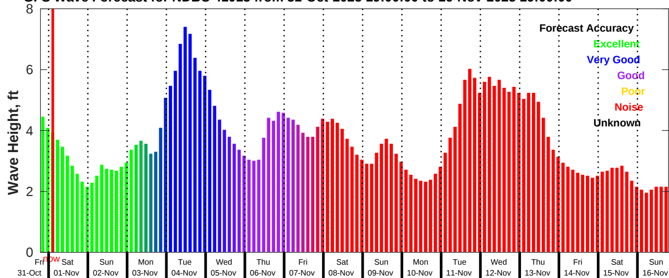
GFS Wave Forecast for NDBC 41013 from 31-Oct-2025 19:00:00 to 16-Nov-2025 19:00:00
