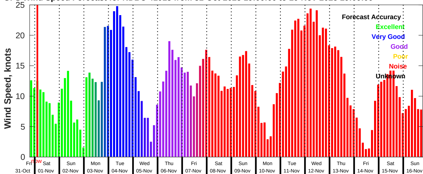
GFS Wind Speed Forecast for NDBC 41013 from 31-Oct-2025 19:00:00 to 16-Nov-2025 19:00:00
