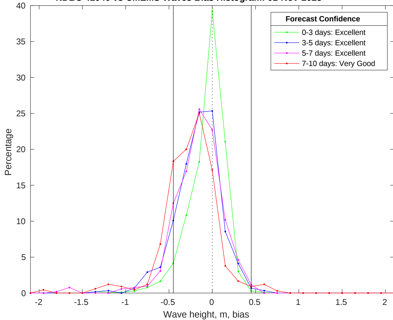
NDBC 41040 vs CMEMS Waves Bias Histogram: 01-Nov-2025
